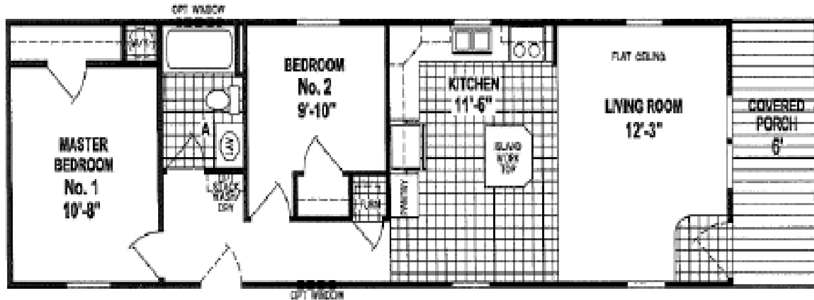
C464C5/5616 (775 SQ. FT.) 1BEDROOM
